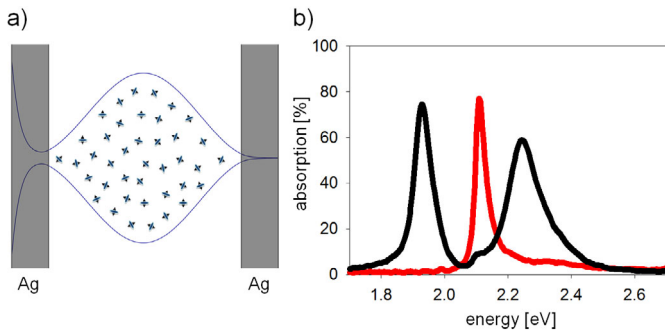
Fig. 1. (a) Illustration of molecules coupled to the fundamental optical mode of a 145 nm thick Fabry-Perot cavity made of two 30 nm thick Ag mirrors. (b) Typical example of absorption spectrum of uncoupled (red line) and coupled (dark line) molecules. The data correspond to J-aggregate (TDBC) molecules dispersed in a polyvinyl alcohol (PVA) polymer host matrix inside the cavity sketched in (a) [27].
