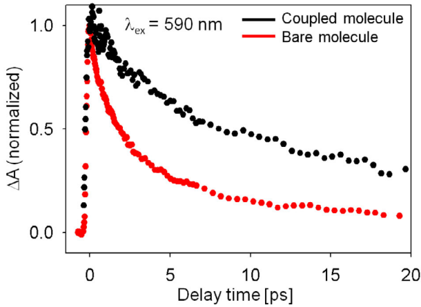
Fig. 4. Temporal evolution of the total change in absorption recorded immediately after a 150 fs pump pulse at 590 nm for a bare film of TDBC molecules (red data) and for TDBC molecules coupled to the cavity (black data; see Fig. 1b). After the pumping rise time, the relaxation appears exponential over this time scale, in agreement with equation (3). The half-life of C^- \sim 4 ps (black) is thus longer than that of the bare molecule (red). At this time scale, the radiative lifetime ( \sim 25 fs) of the low Q cavity appears as instantaneous.
