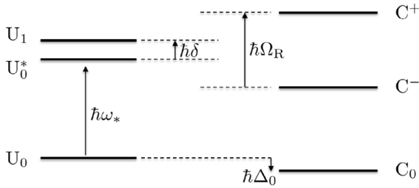
Fig. 2. Energy diagram of the bare states U and dressed states C of the “molecule+cavity” system. The energy difference between U_1 and U_0^* is \hbar\delta , with \delta = \omega_1 - \omega_* the detuning between the frequency \omega_1 of the cavity mode, and \omega_* that of the molecular transition. The Rabi splitting \hbar\Omega_R between the dressed states C^+ and C^- and the energy shift \hbar\Delta_0 of the ground state C_0 are shown.
