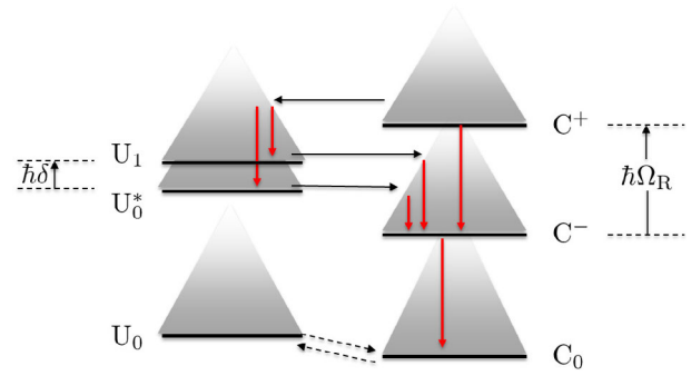
Fig. 3. Schematic representation of uncoupled U and coupled C states in the non-Markovian regime. The vibrational ladders associated with each molecular configuration are represented in grey shadows and the non-radiative relaxation paths as red vertical arrows. Transitions occurring between uncoupled and coupled molecules are represented by horizontal black arrows.
